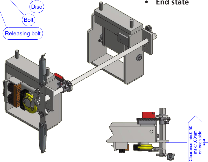
Detail reversing lever / actuating shaft
